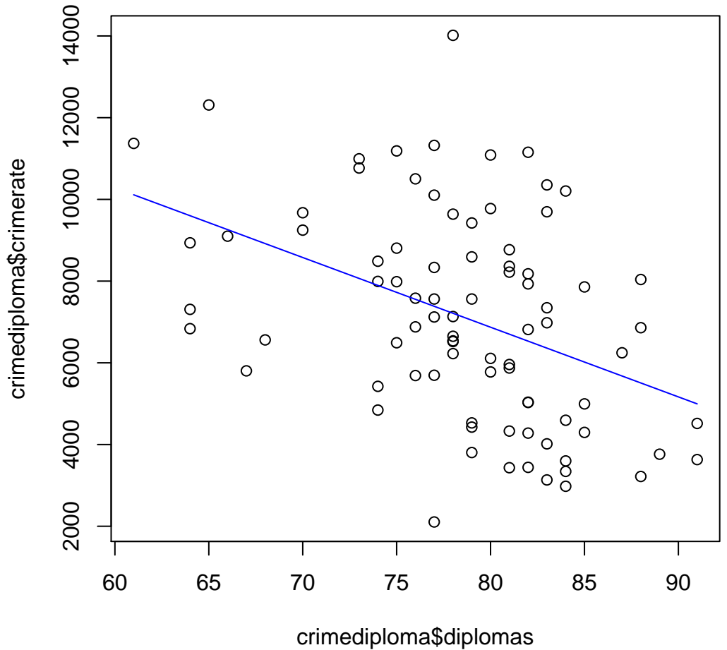
scatter plot
