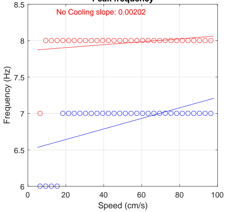
Peak frequency
