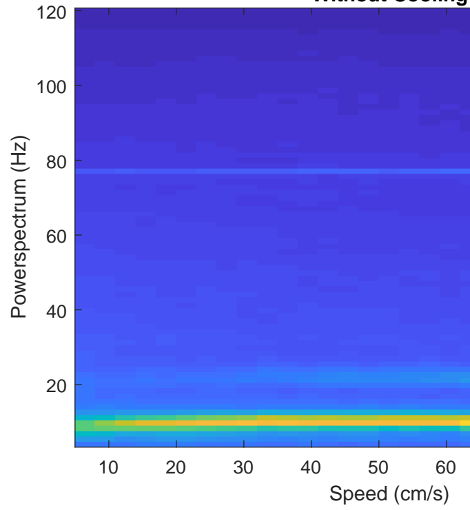
Without Cooling
