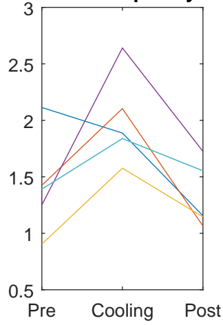
Oscillation Frequency-theta
