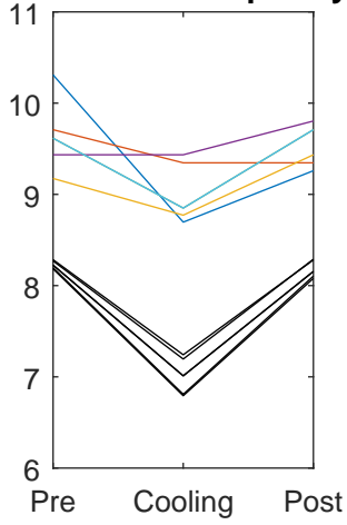
Oscillation Frequency
