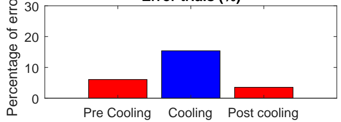
Error trials (%)
