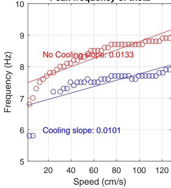
Peak frequency of theta
