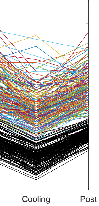
Oscillation Frequency
