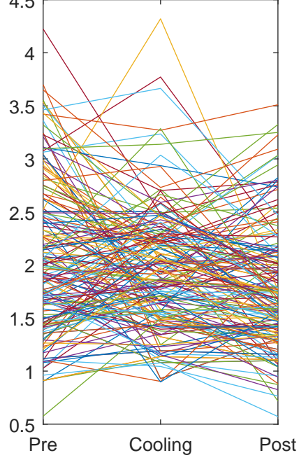
Oscillation Frequency-theta
