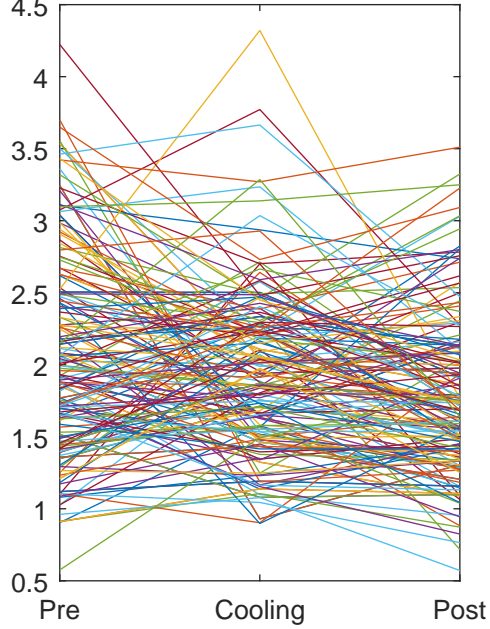
Oscillation Frequency-theta
