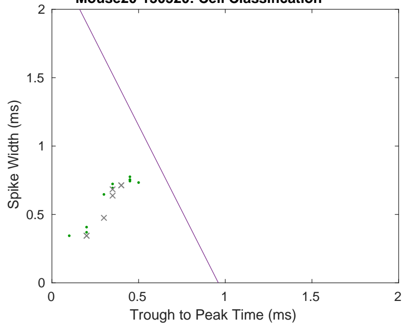
Mouse20-130520: Cell Classification
