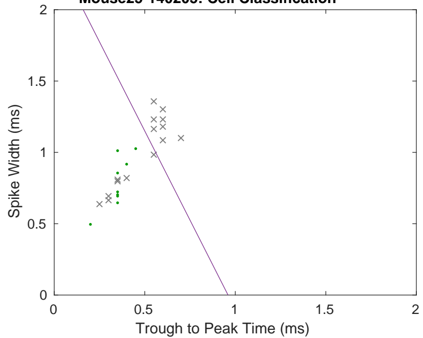
Mouse25-140205: Cell Classification
