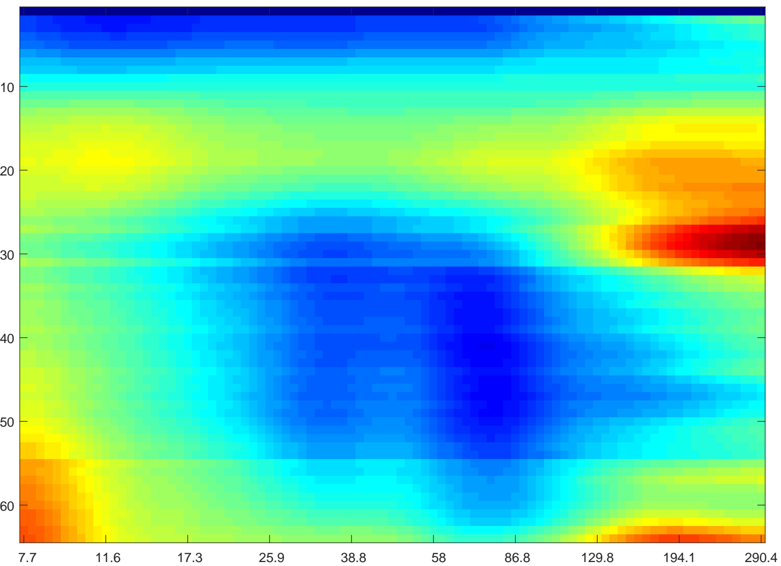
YMV09_171204--wavelet-depth-profile-WAKE--8-300Hz
