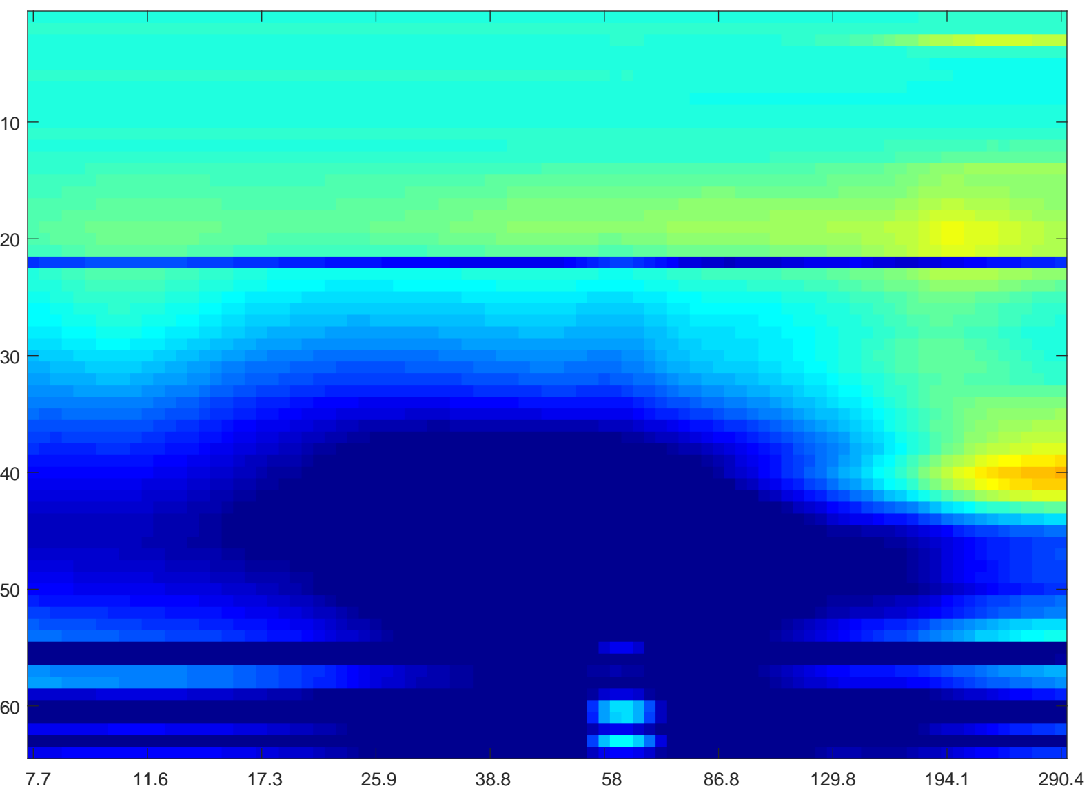
YMV10 1 71213--wavelet-depth-profile-NREM--8-300Hz
