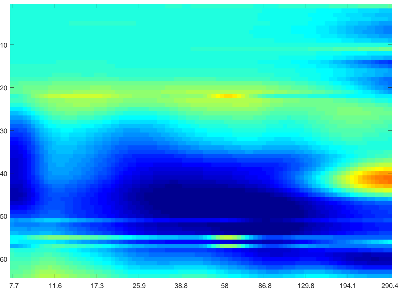
YMV11 1 71208--wavelet-depth-profile-NREM--8-300Hz
