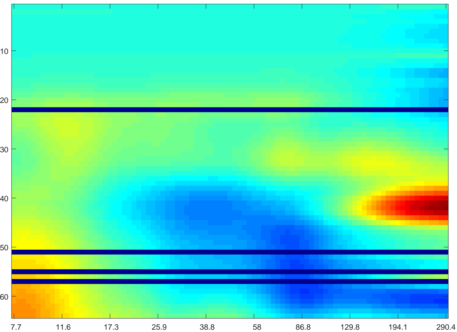
YMV11 1 71208--wavelet-depth-profile-WAKE--8-300Hz
