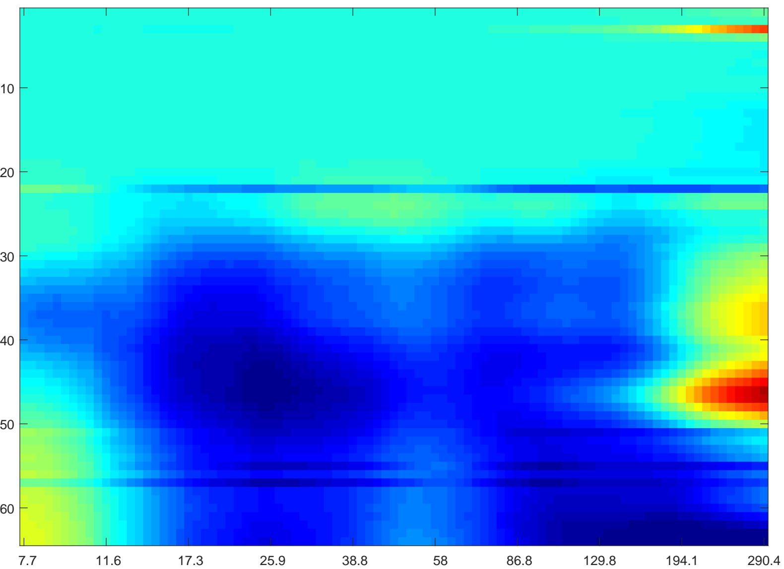
YMV12 1 71211--wavelet-depth-profile-REM--8-300Hz
