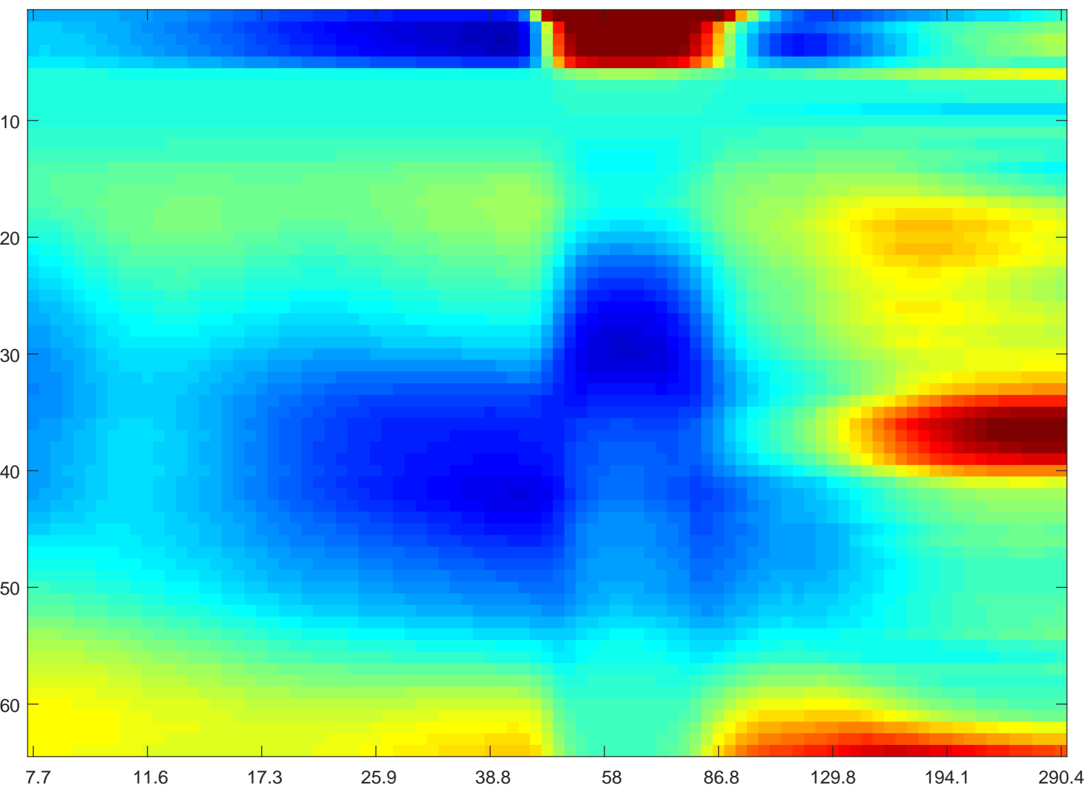
YMV13 1 80127--wavelet-depth-profile-NREM--8-300Hz
