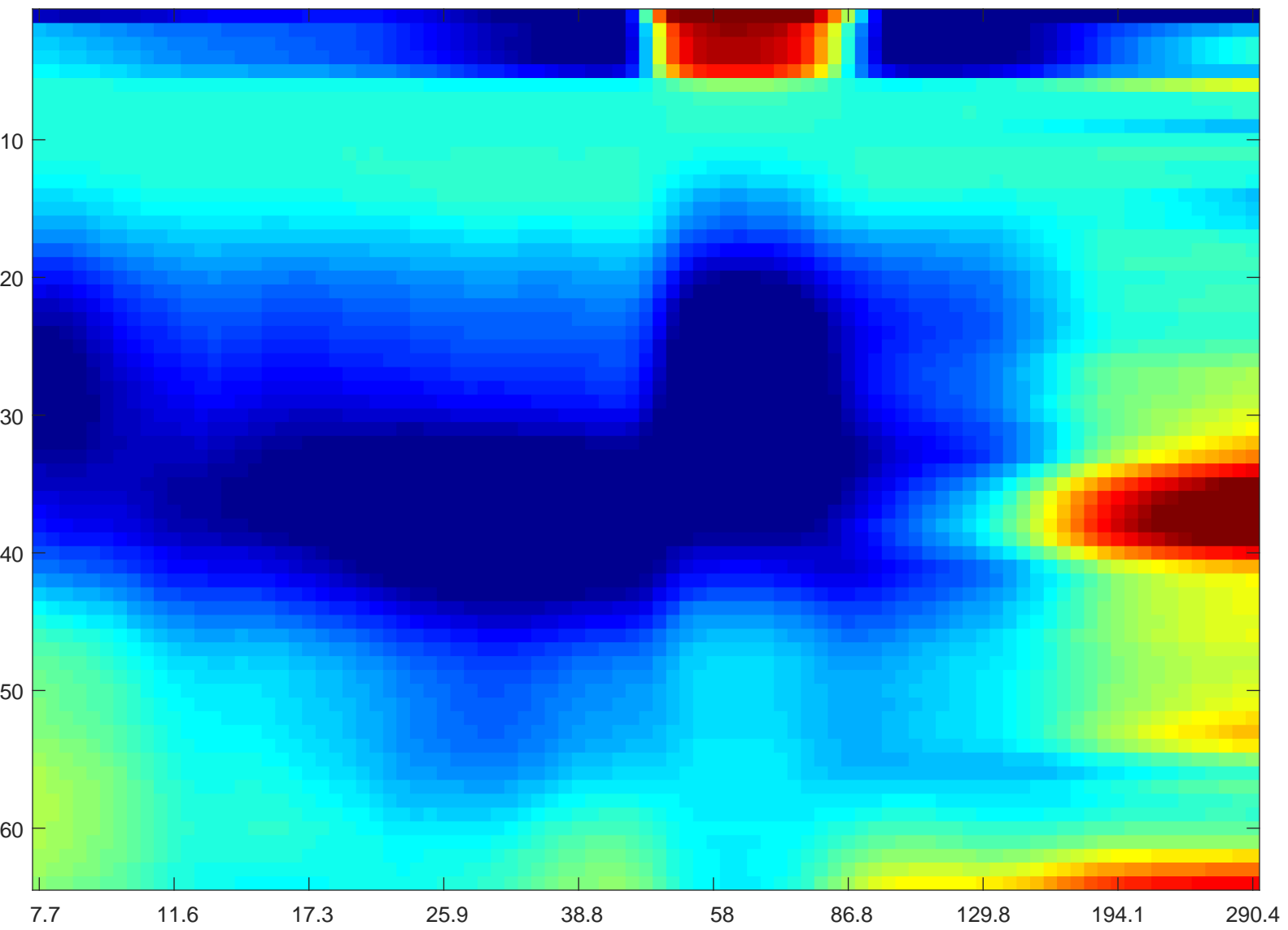
YMV13 1 80127--wavelet-depth-profile-REM--8-300Hz
