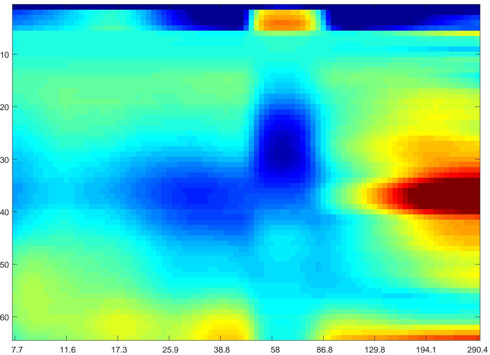
YMV13 1 80127--wavelet-depth-profile-WAKE--8-300Hz
