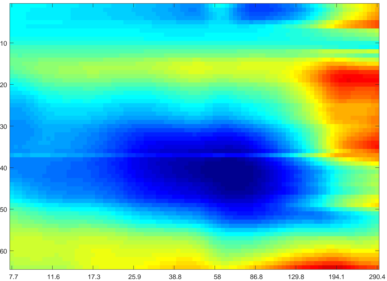
YMV14 1 80128--wavelet-depth-profile-NREM--8-300Hz
