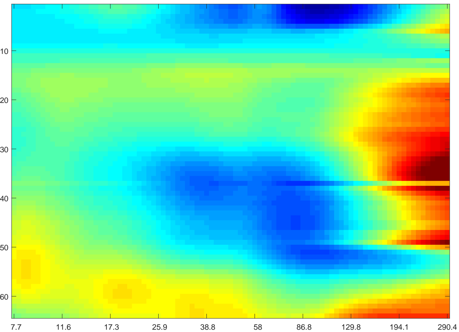
YMV14_180128--wavelet-depth-profile-WAKE--8-300Hz
