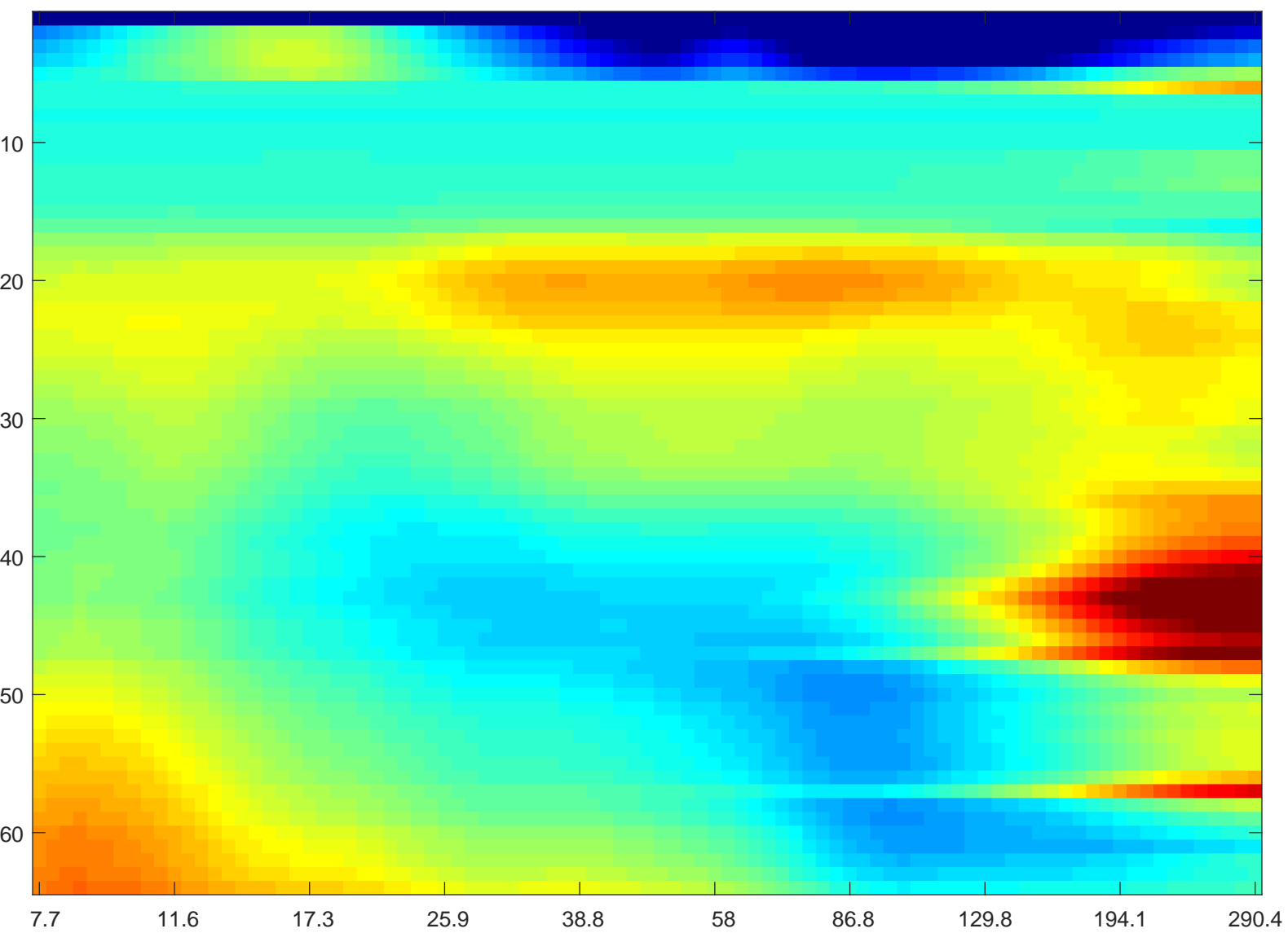
YMV15 1 80205--wavelet-depth-profile-WAKE--8-300Hz
