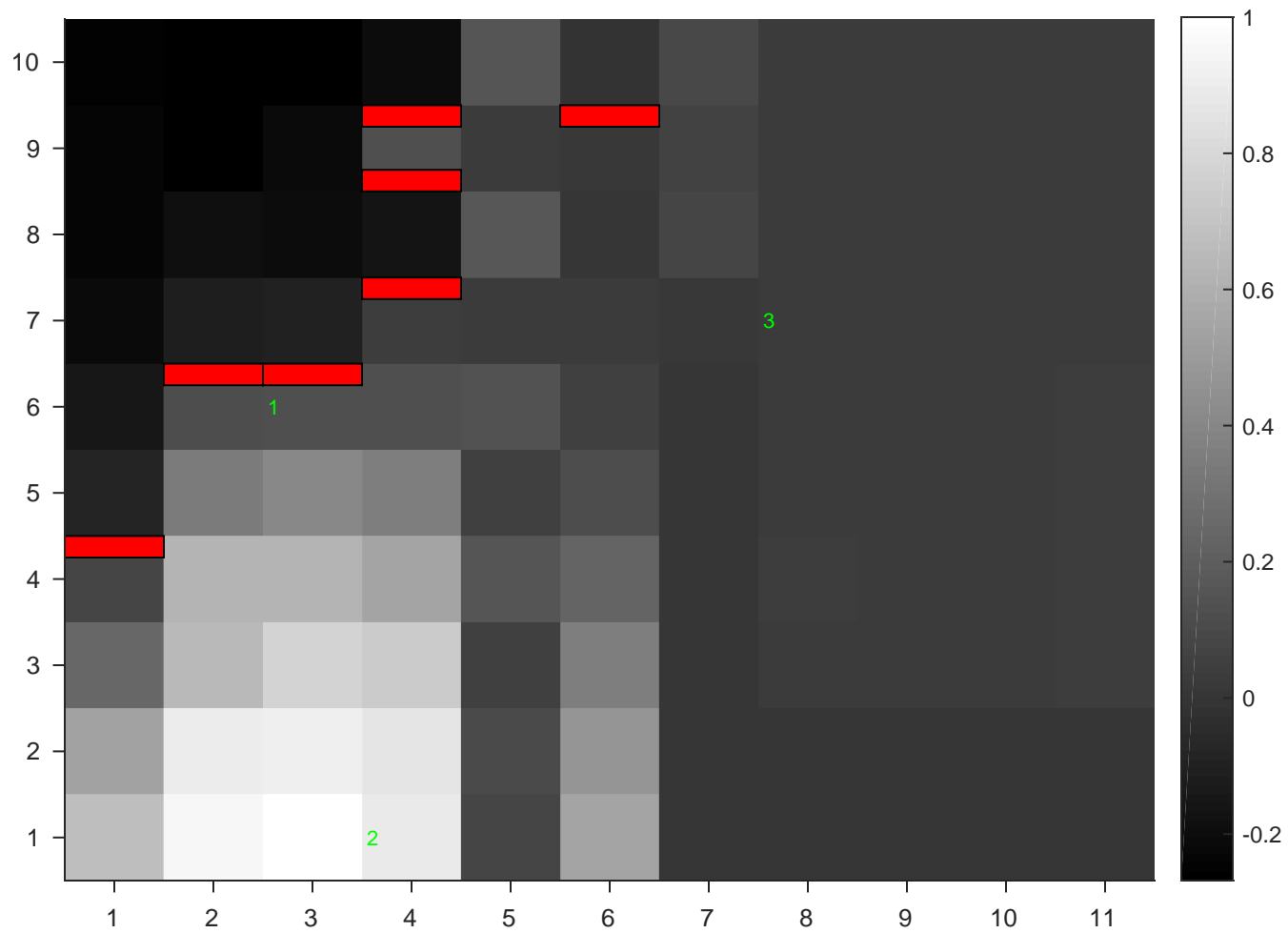
YutaMouse32-150317--DS2map-trigCh28w u nits
