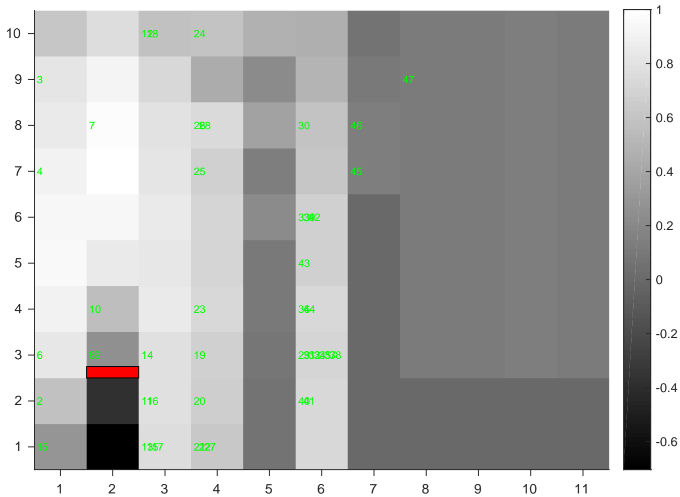
YutaMouse32-150323--DS2map-trigCh42w u_nits
