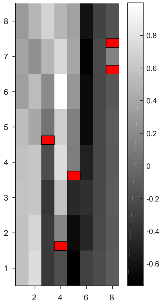
YutaMouse39-150803--DS2map _mV-trigCh26
