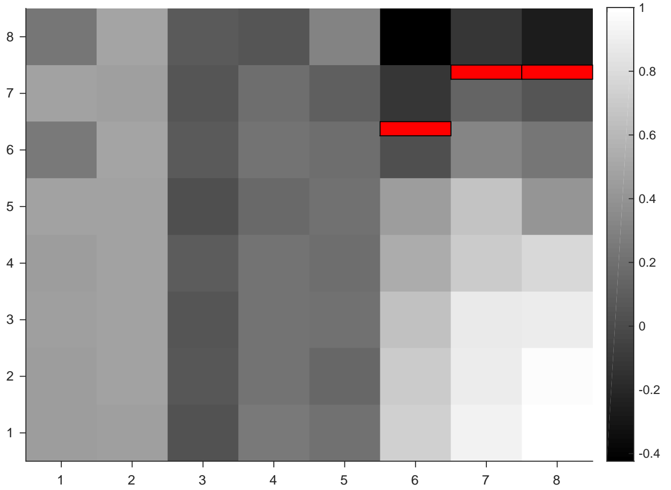
YutaMouse42-151105--DS2map-trigCh60
