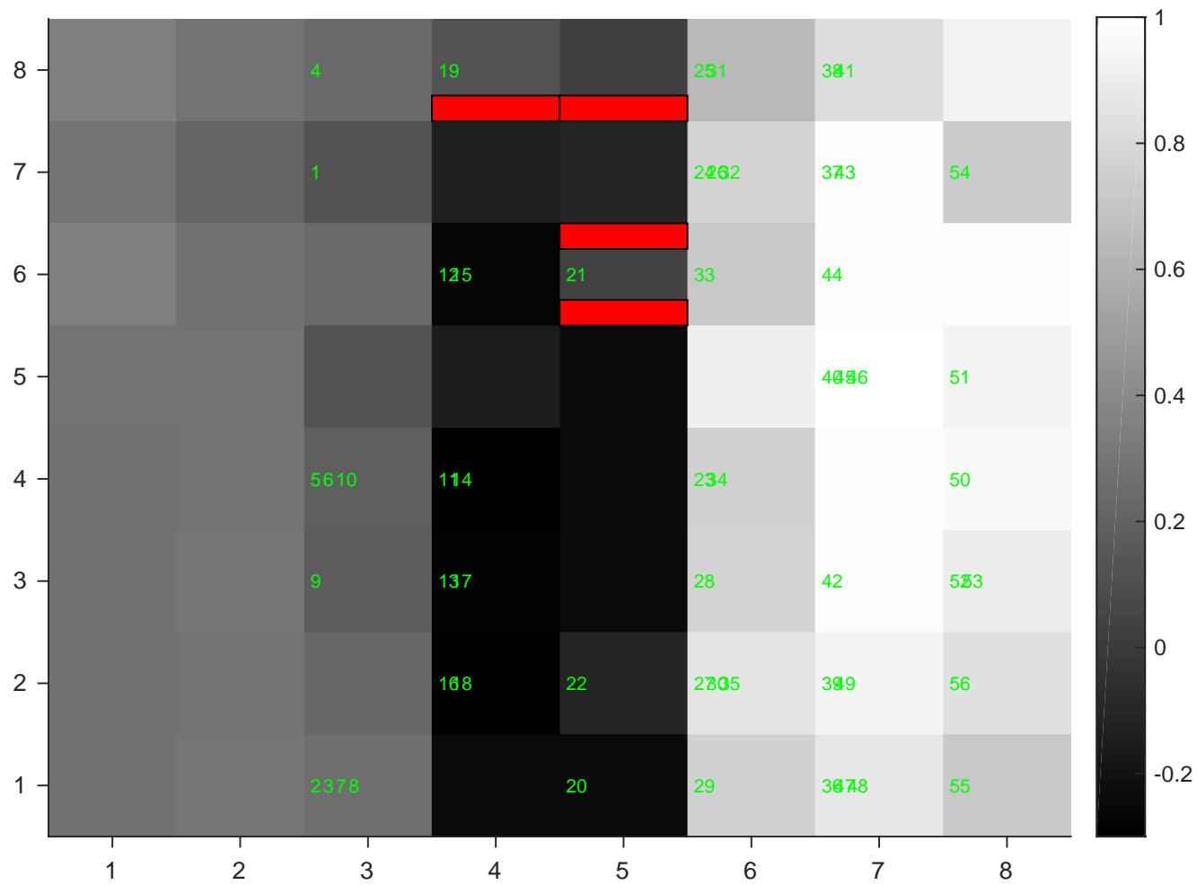
YutaMouse42-151108--DS2map-trigCh10w u_nits
