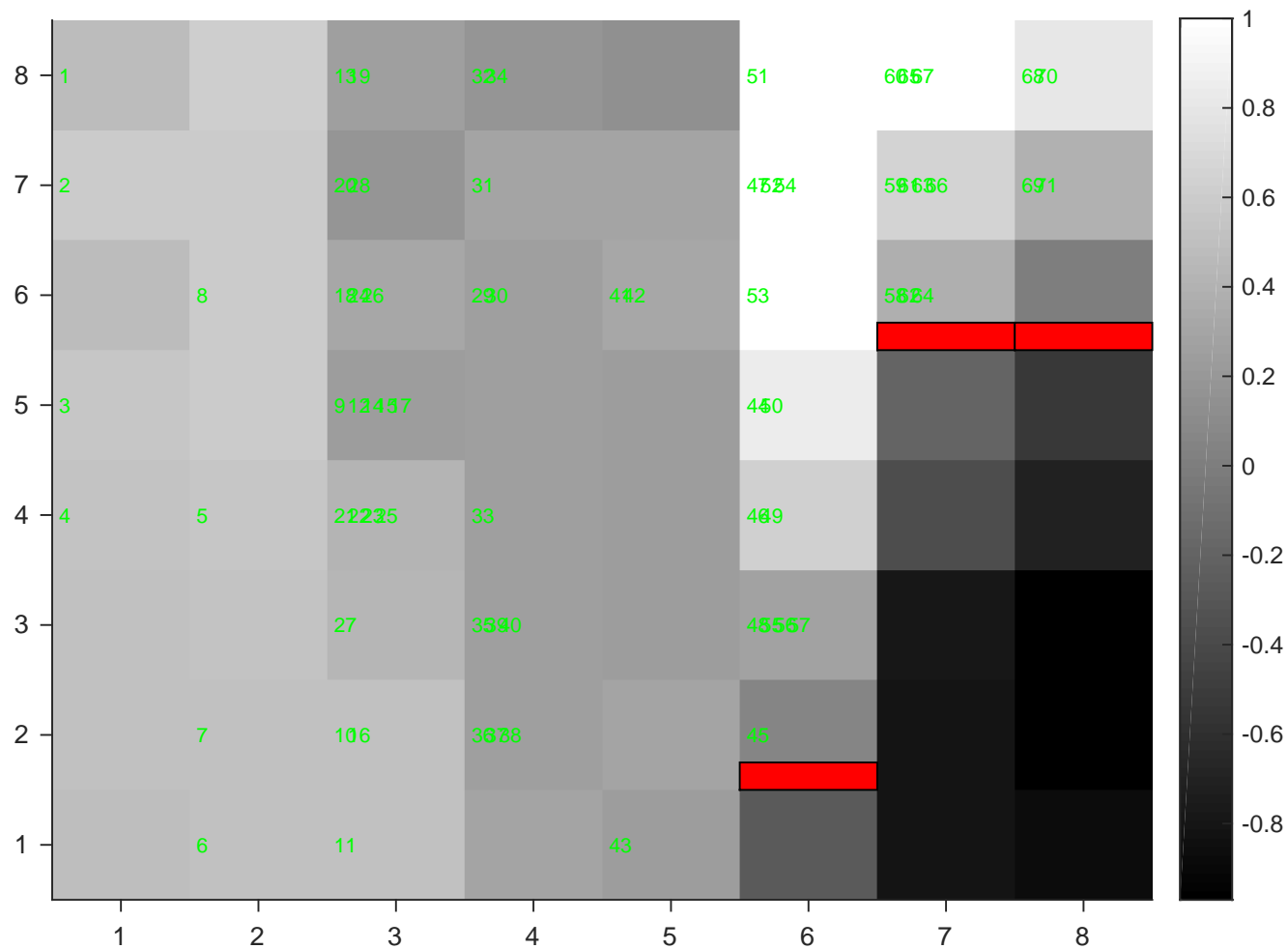
YutaMouse42-151111--DS2map-trigCh56w u_nits
