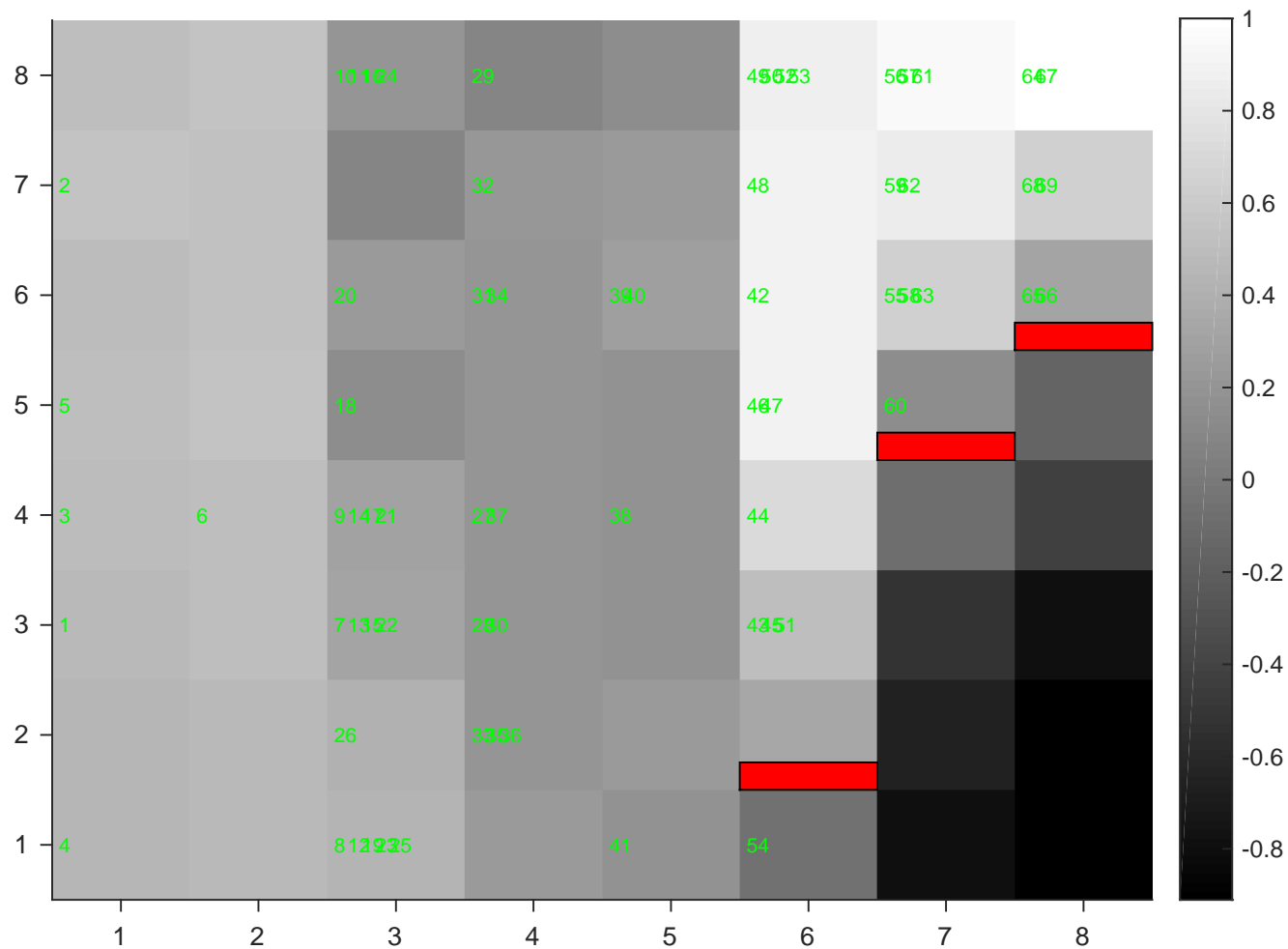
YutaMouse42-151113--DS2map-trigCh56w units
