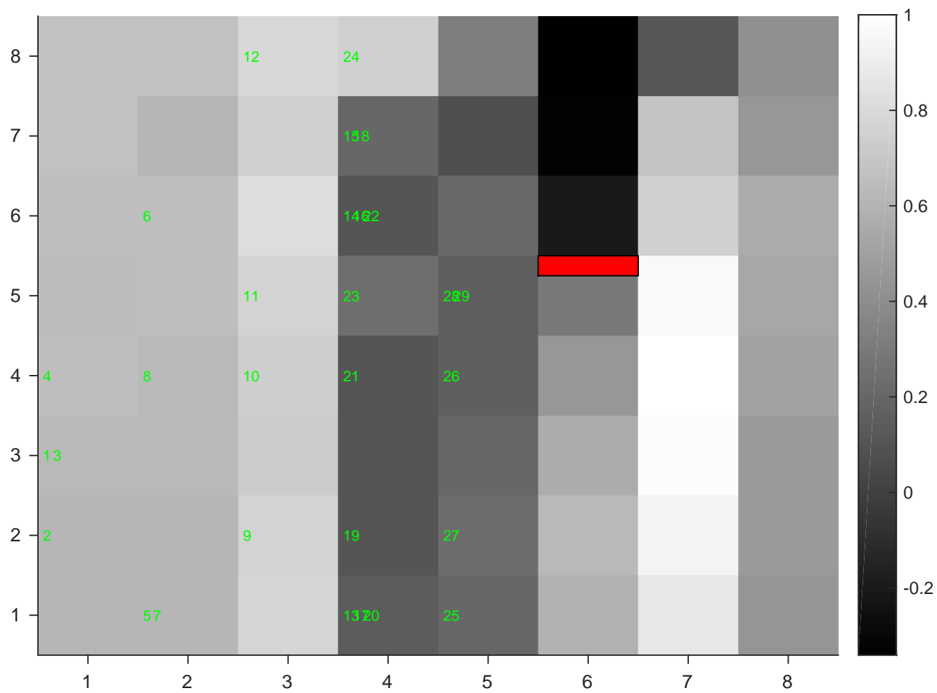
YutaMouse42-151118--DS2map-trigCh53w u_nits
