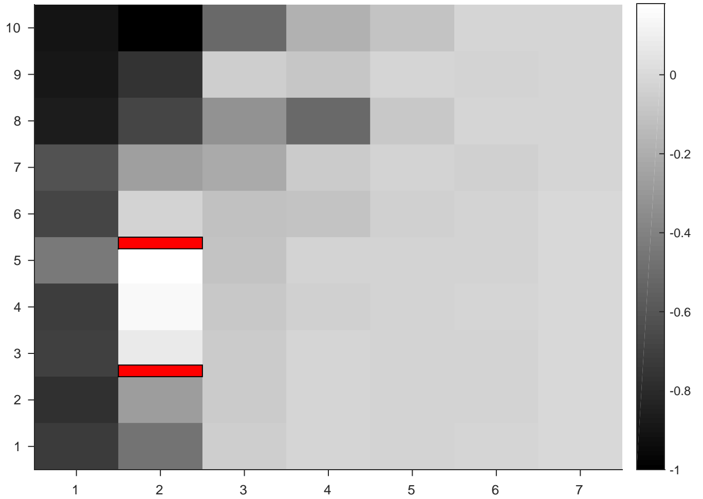
YutaMouse44-151129--DS2map-trigCh17
