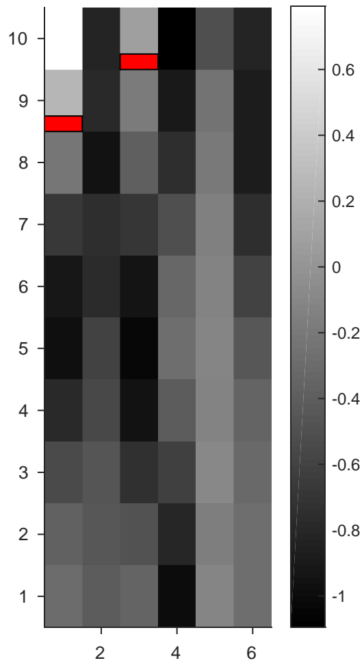
YutaMouse51-160516--DS2map _mV-trigCh33
