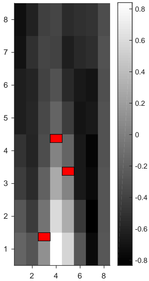
YutaMouse54-160630--DS2map _mV-trigCh31
