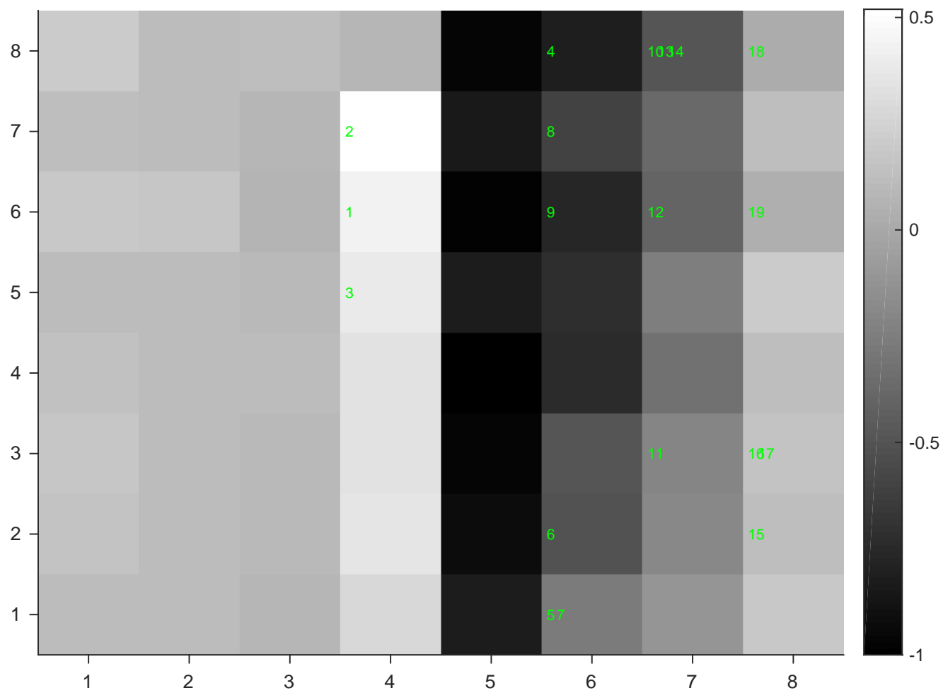
YutaMouse55-160908--DS2map-trigCh62w u_nits
