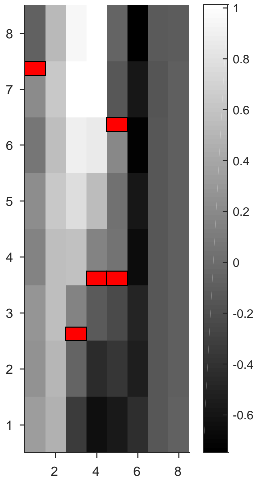
YutaMouse56-160911--DS2map _mV-trigCh26
