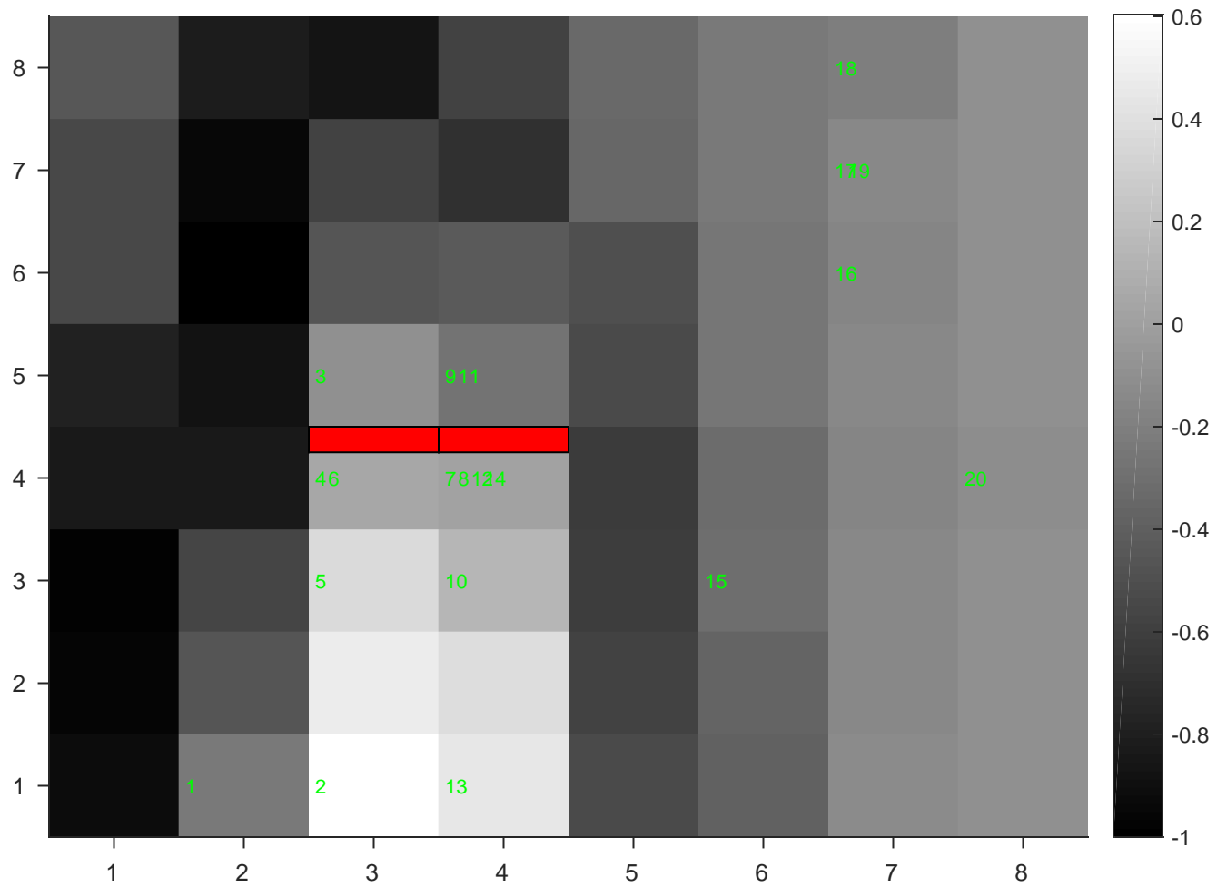
YutaMouse56b160913--DS2map-trigCh21w \mu nits
