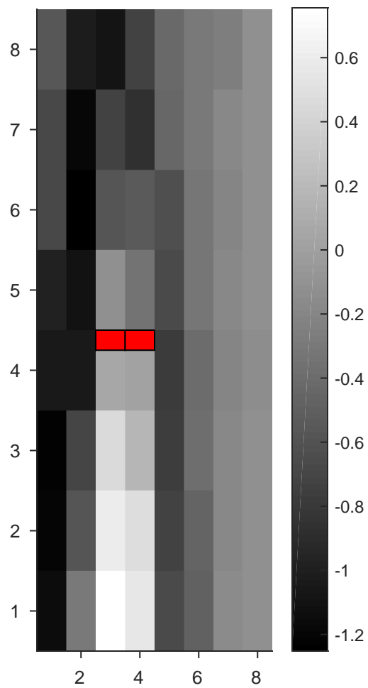
YutaMouse56b160913--DS2map _mV-trigCh21
