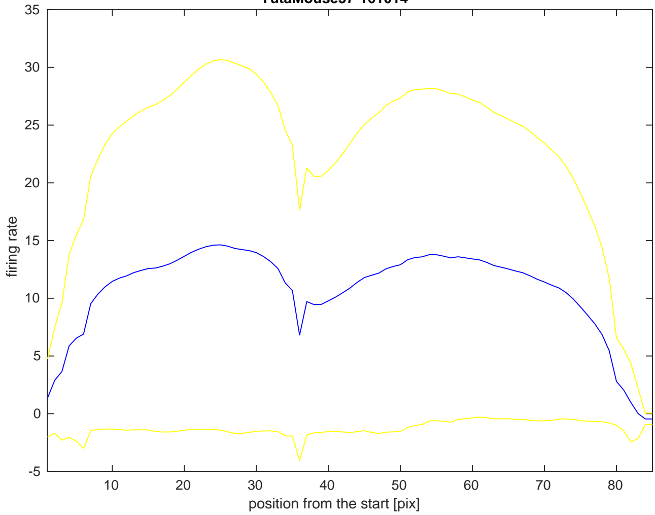
YutaMouse57-161014--velocity-on-figure-eight-maze YutaMouse57-161014
