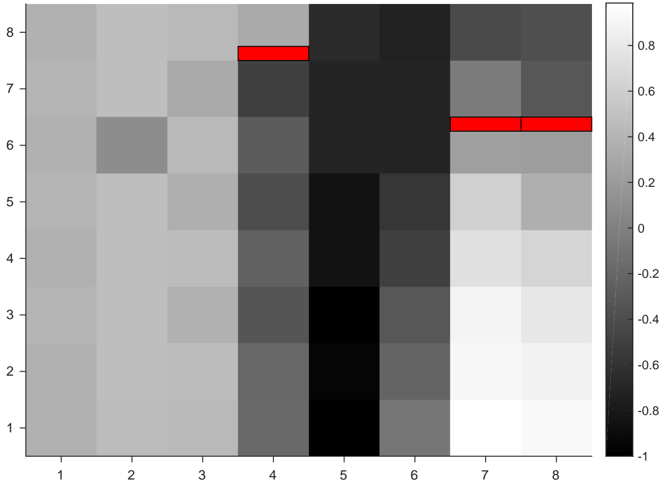
YutaMouse59-170214--DS2map-trigCh60
