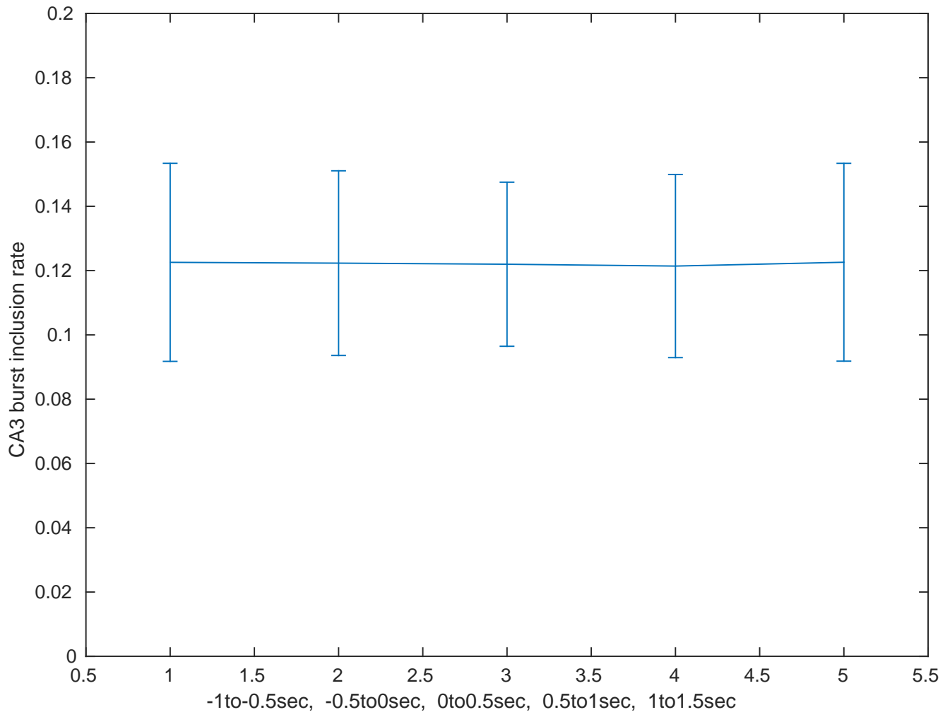
YutaMouse59-170214--ca3burst-amplitude--POMC-stim
