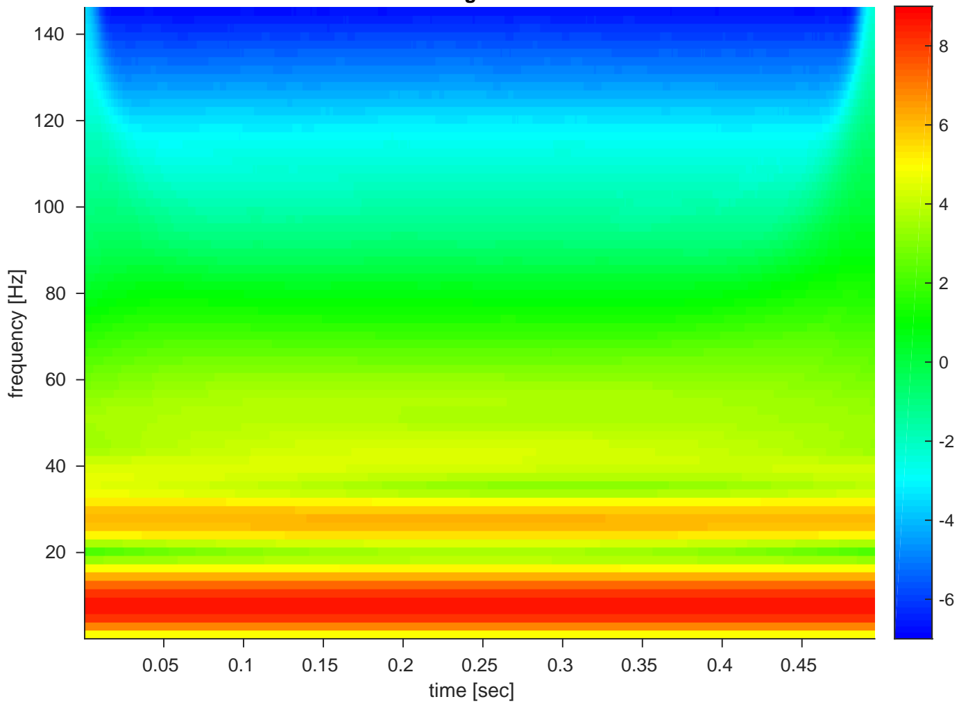
YutaMouse59-170214--wavelet-during-POMC-stim during stim
