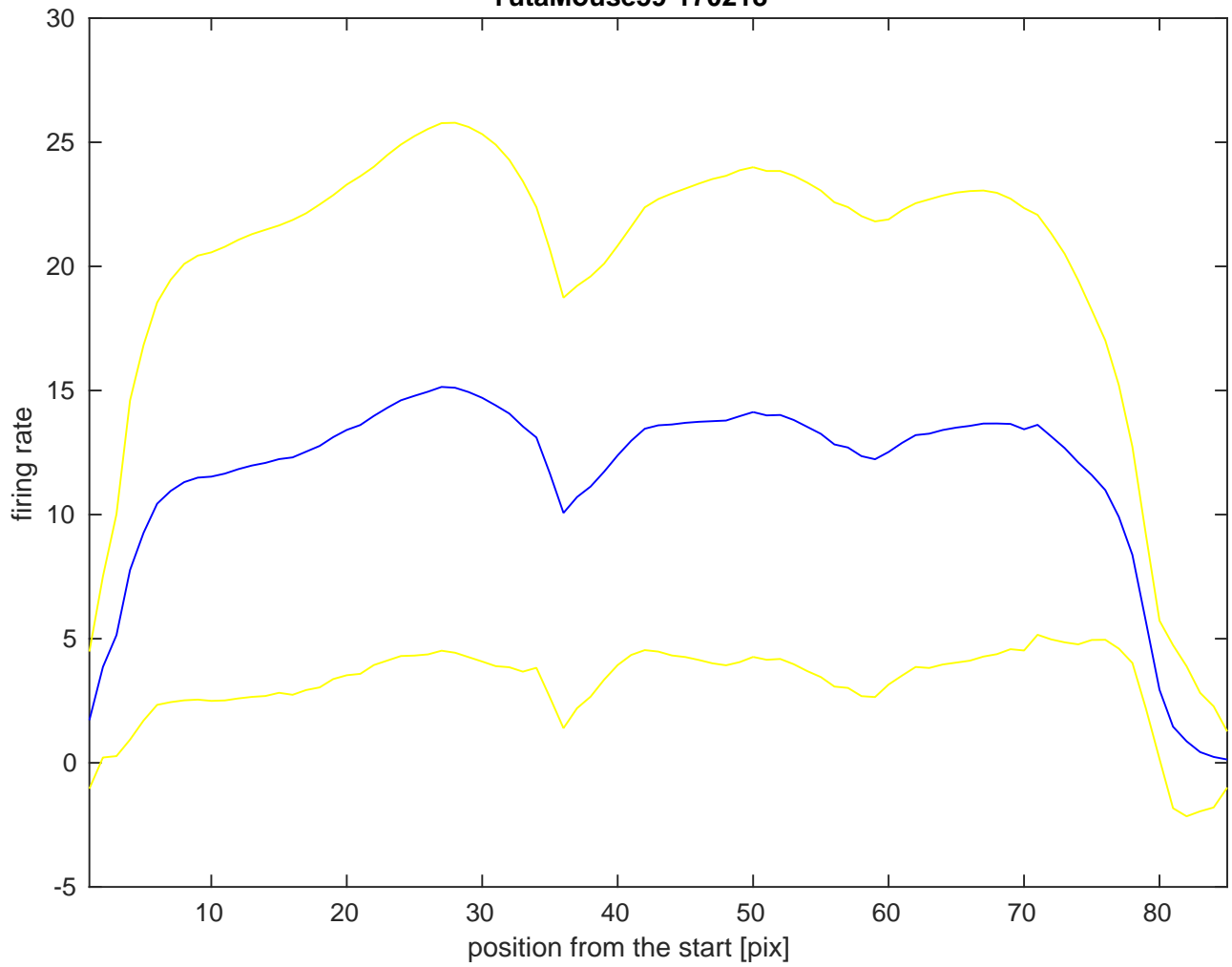
YutaMouse59-170218--velocity-on-figure-eight-maze YutaMouse59-170218
