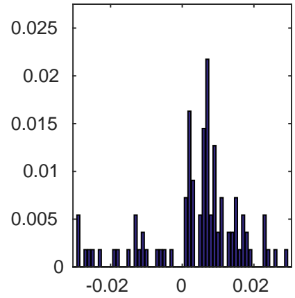
burst 1st spike
