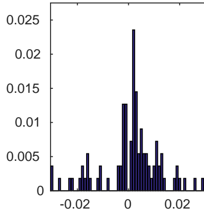
burst 2nd spike
