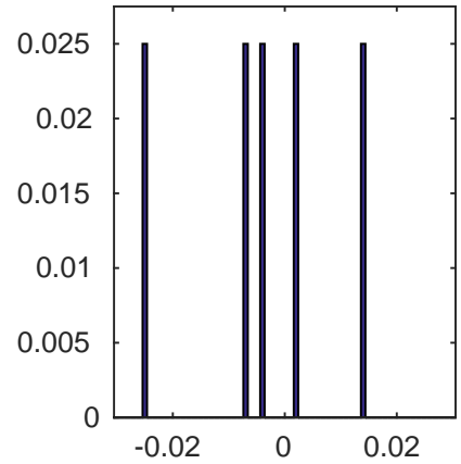
burst 3rd spike
