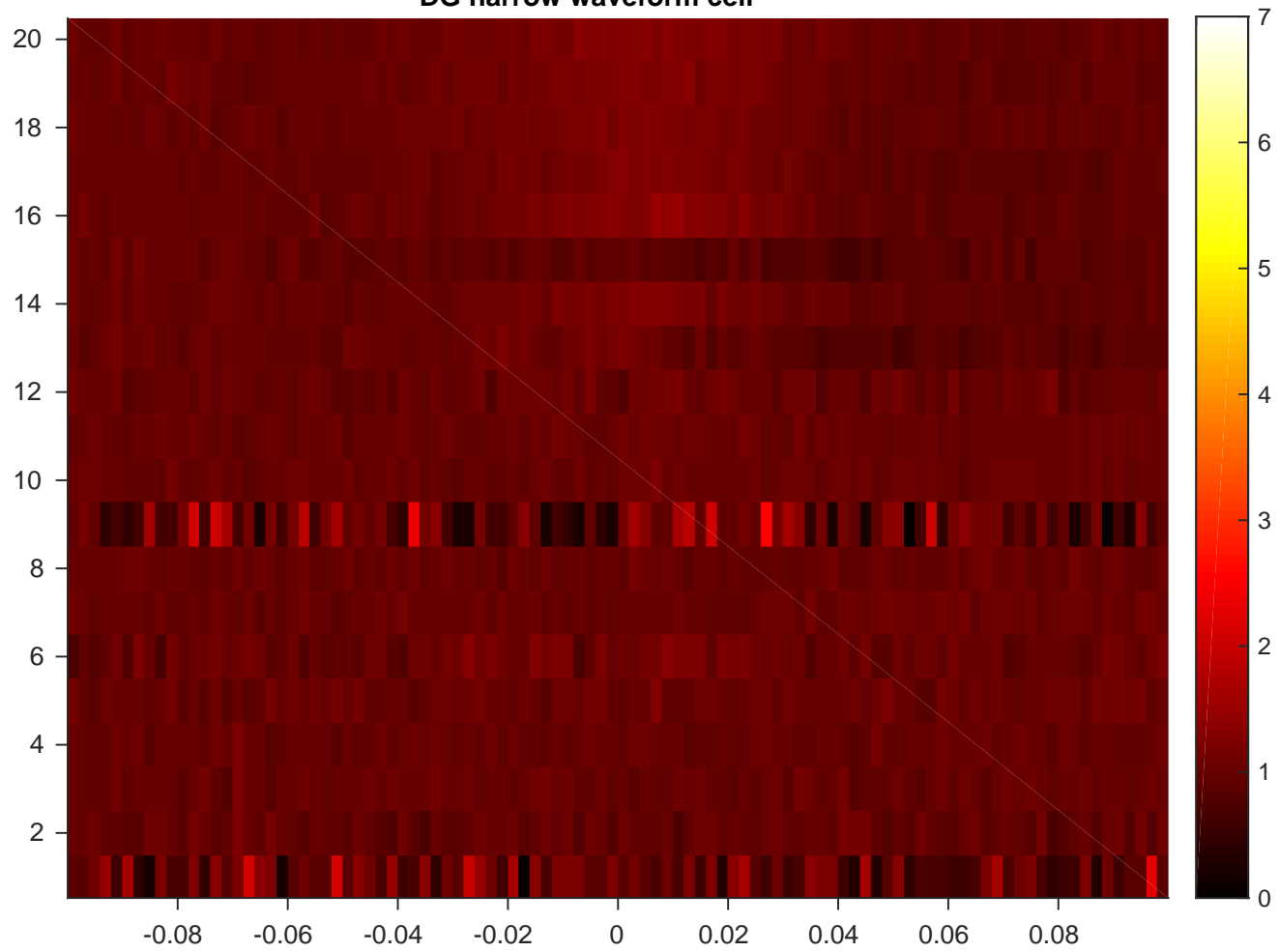
DG a II 5 --DG narrow waveform cell--CA3burstpeakAligned DG narrow waveform cell
