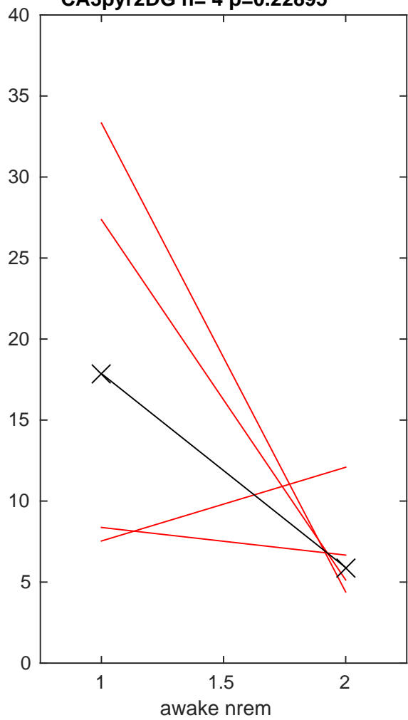
DG a II 5 --SpikeTransmission--Awake-NREM--CA3pyr2DG--median CA3pyr2DG n= 4 p=0.22895
