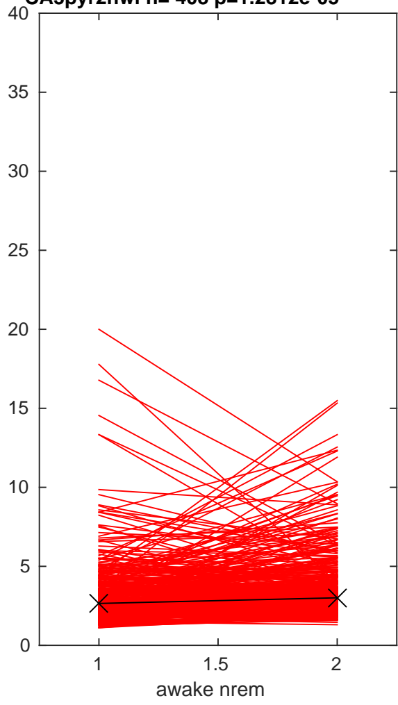
DG a5 II --SpikeTransmission--Awake-NREM--CA3pyr2nwi--median CA3pyr2nwi n= 408 p=1.2812e-05
