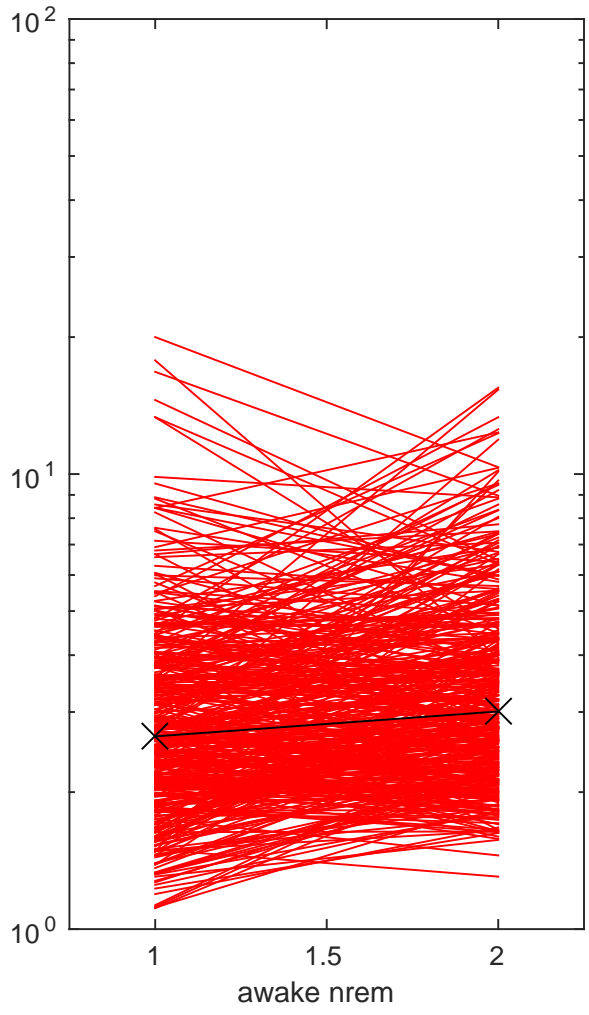
DG a5 II --SpikeTransmission--Awake-NREM--CA3pyr2nwi--median CA3pyr2nwi n= 408 p=1.2812e-05
