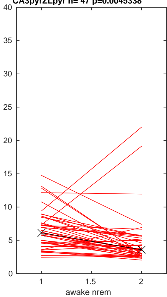
DG a II 5 --SpikeTransmission--Awake-NREM--CA3pyrZLpyr--median CA3pyrZLpyr n= 47 p=0.0045338
