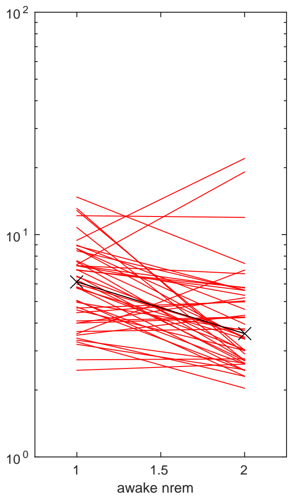
DG a II 5 --SpikeTransmission--Awake-NREM--CA3pyrZLpyr--median CA3pyrZLpyr n= 47 p=0.0045338
