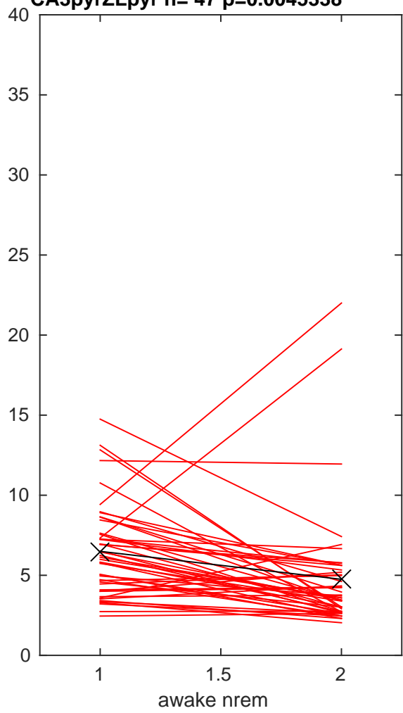
DG a5 --SpikeTransmission--Awake-NREM--CA3pyrZLpyr CA3pyrZLpyr n= 47 p=0.0045338
