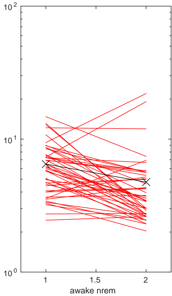
DG a5 --SpikeTransmission--Awake-NREM--CA3pyrZLpyr CA3pyrZLpyr n= 47 p=0.0045338
