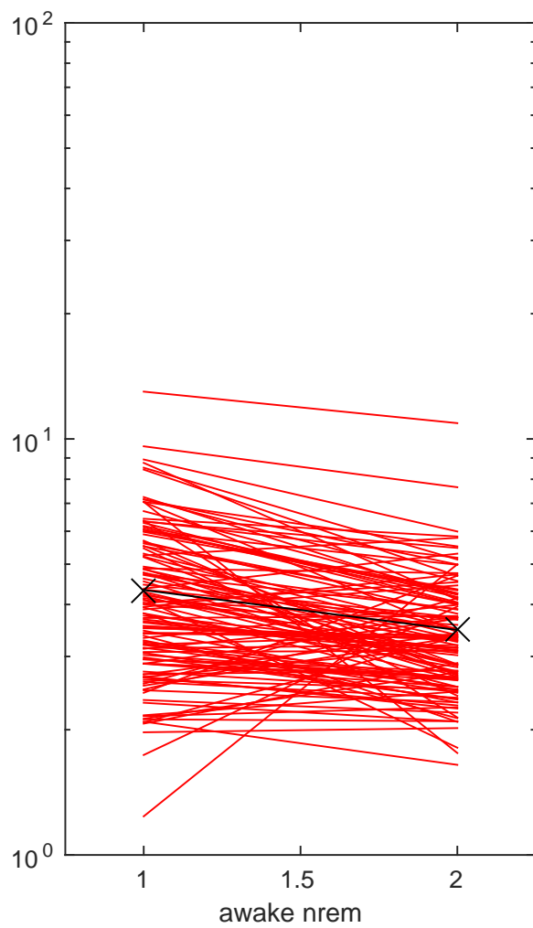
DG a5 II --SpikeTransmission--Awake-NREM--gra2nwi gra2nwi n= 120 p=4.428e-10
