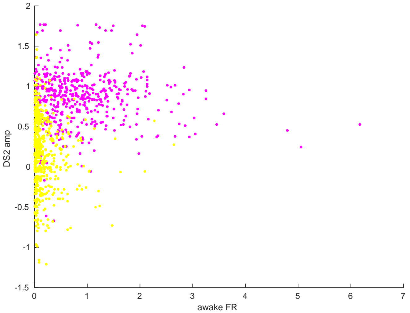
DG a II 5 --WaveformGranuleVsMossy-final--parameters-all-awakeFR-vs-DS2amp
