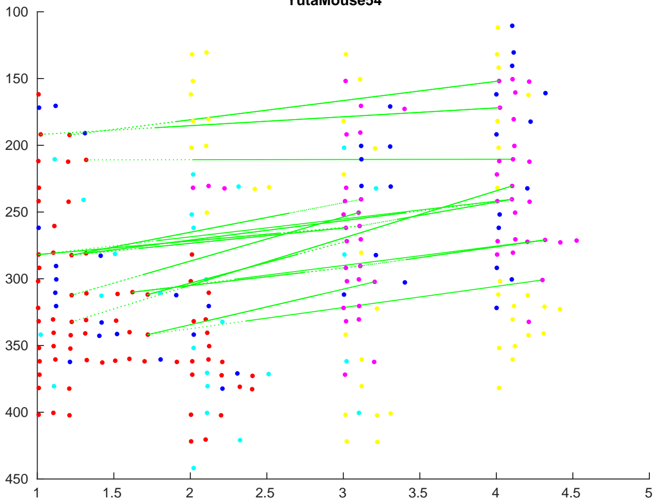
DG a II 5 --YutaMouse54--EEinteractionMap--onlyZeroLag--direction YutaMouse54
