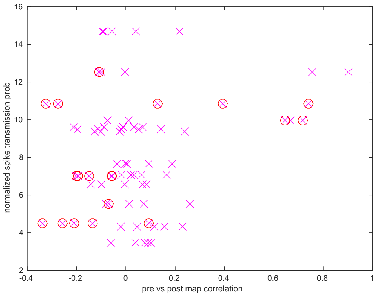
DG a II 5 --gravsmos-prevspost-open-fields--corr-vs-normSpkTrans--all
